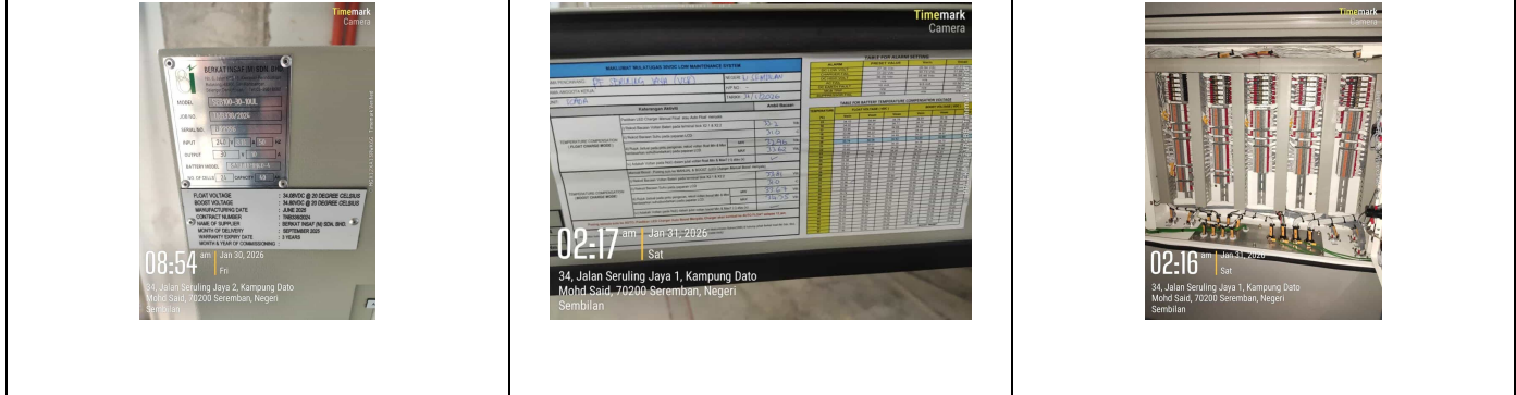
BATTERY CHARGER (COMPLETE WARRANTY STICKER) OVERVIEW OF BATTERY CHARGER (COMPLETE WITH 30VDC LOW MAINTENANCE SYSTEM COMMISSIONING CHECKLIST) INSIDE BATTERY CHARGER INDIVIDUAL EARTHING CONNECTIONS COMPLETED FOR I/O CABLES TO EARTH STUD AT RCB PANEL
